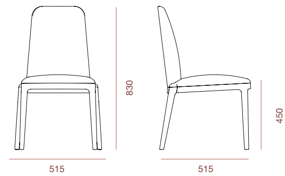
HIGH BACK CHAIR
