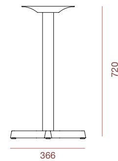
SMALL TABLE BASE
